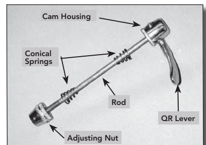
Fig. 2: Front QR anatomy shown properly assembled.
